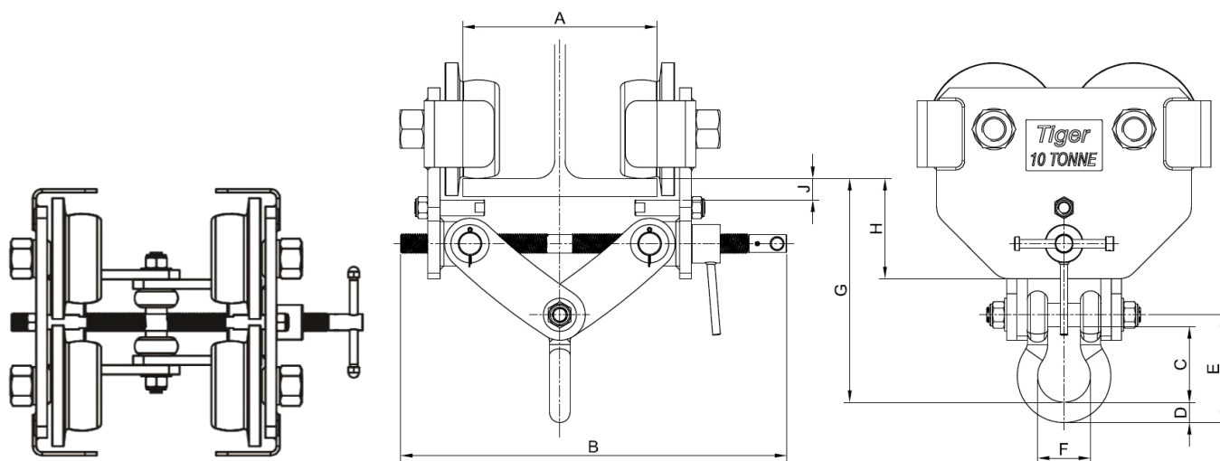
10t Adjustable Plain Trolley (APT)
